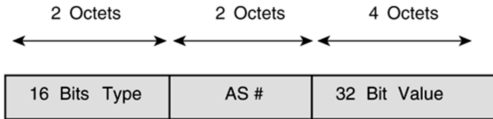
Figure 10-7. BGP Extended Community Attribute Format
